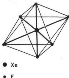
Figure 10 "First guess" structure for \text{XeF}_6 .
