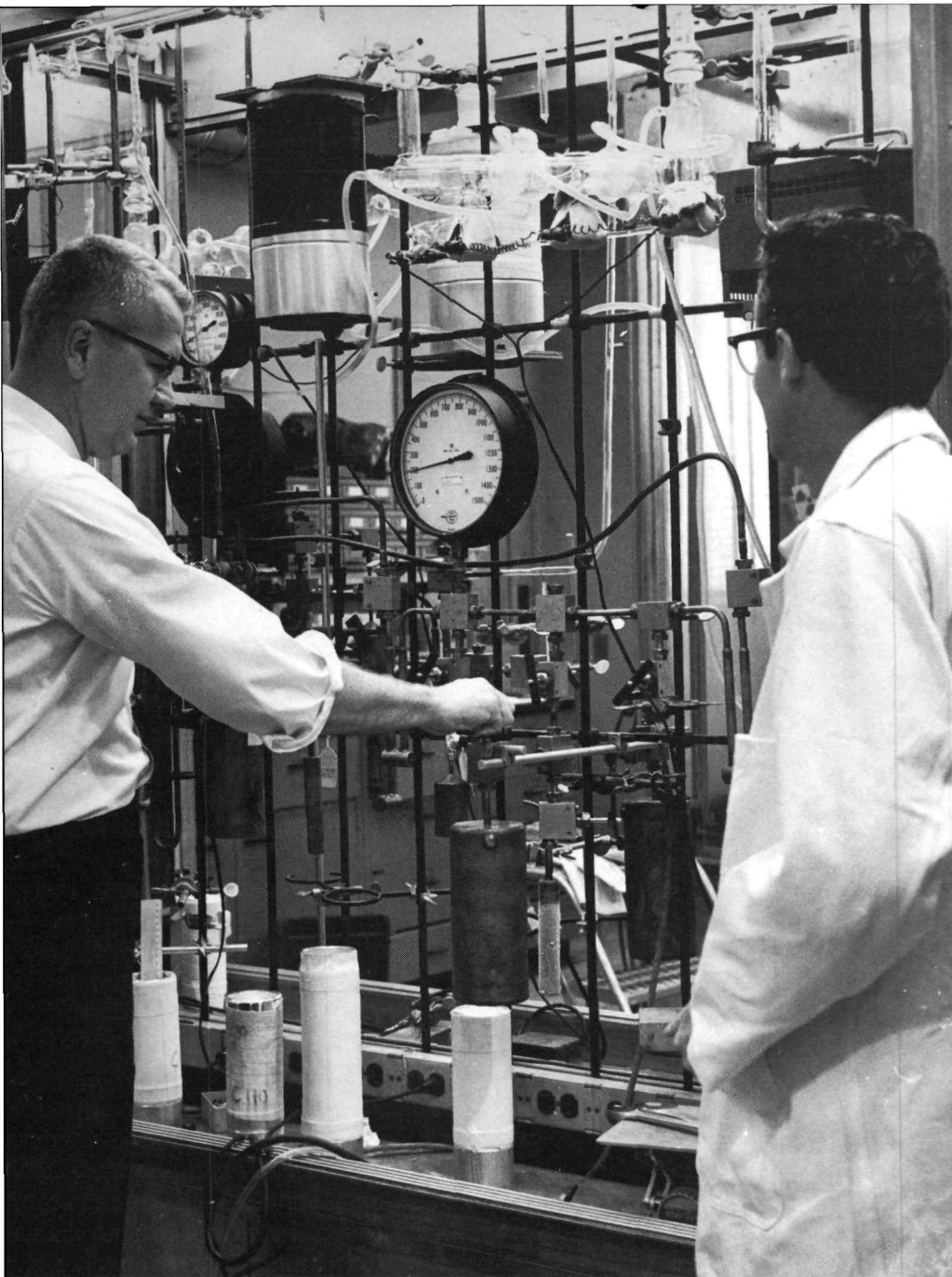
Figure 6 John G. Malm (left) and Howard H. Claassen adjusting apparatus similar to that used for the first preparation of \text{XeF}_4 at Argonne National Laboratory.
